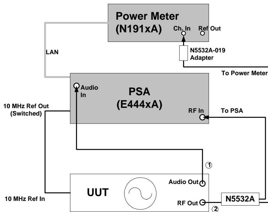
Figure 2-1 Hardware Setup Block Diagram
