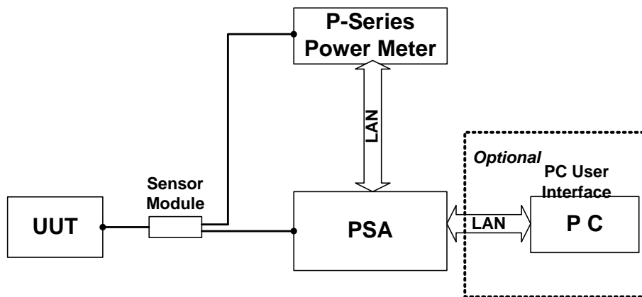
Figure 5-1 N5531S Block Diagram
