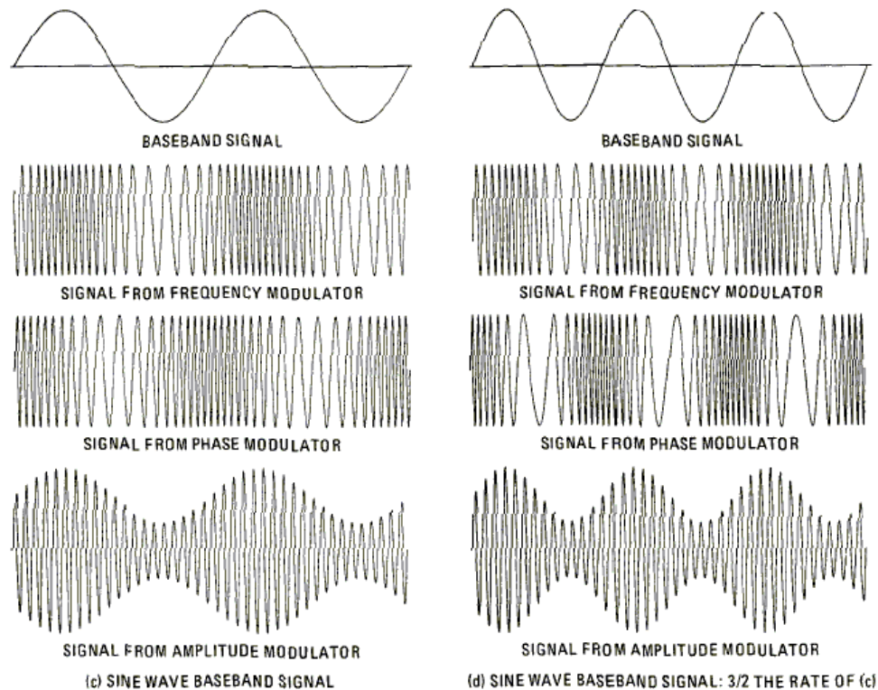
Figure 5-9 Signals from Frequency, Phase and Amplitude Modulators for Various Baseband Signals (Sine Waves)
