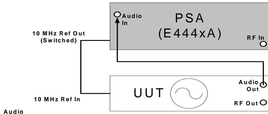
Figure 3-23 Audio Test Connection Diagram
