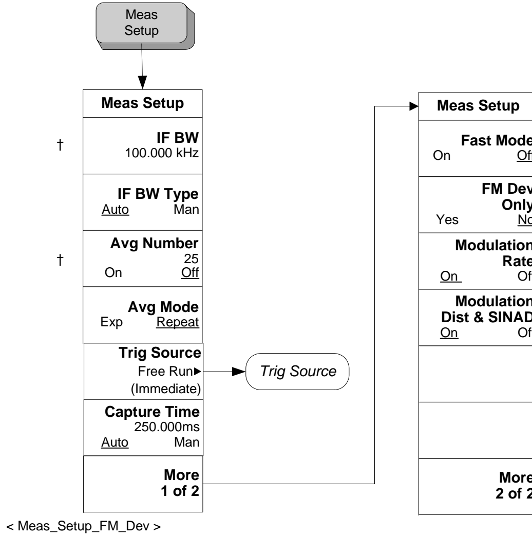
Figure 6-17 FM Deviation Measurement Setup Key Flow
