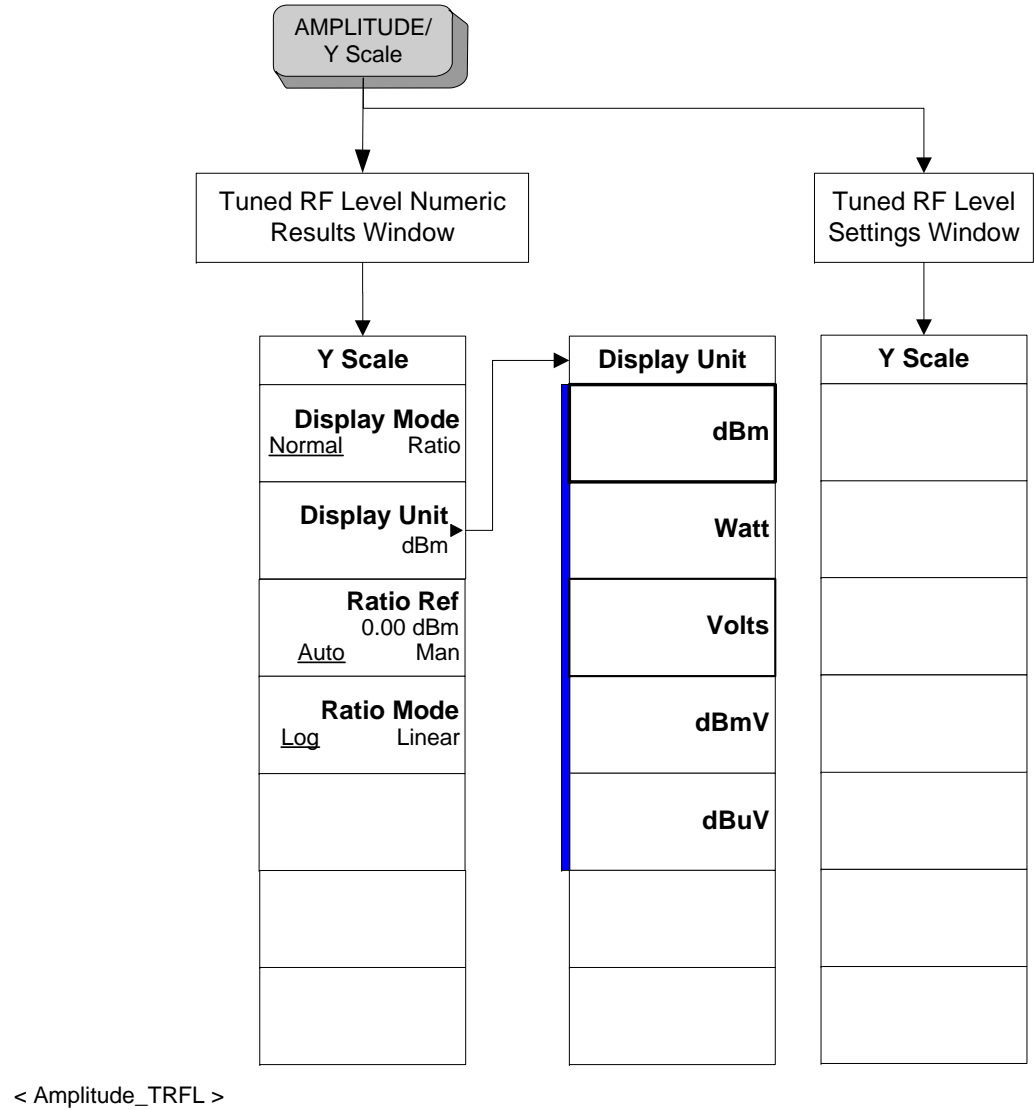
Figure 6-45 TRFL Amplitude Selection Key Flow
