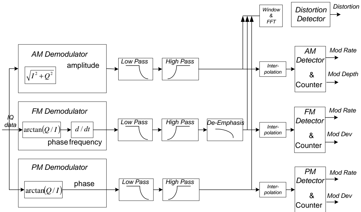
Figure 5-11 Demodulation Diagram
