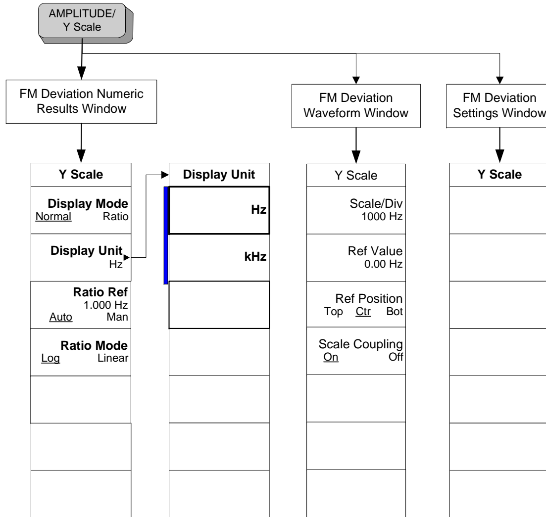
Figure 6-34 PM Deviation Amplitude Selection Key Flow
