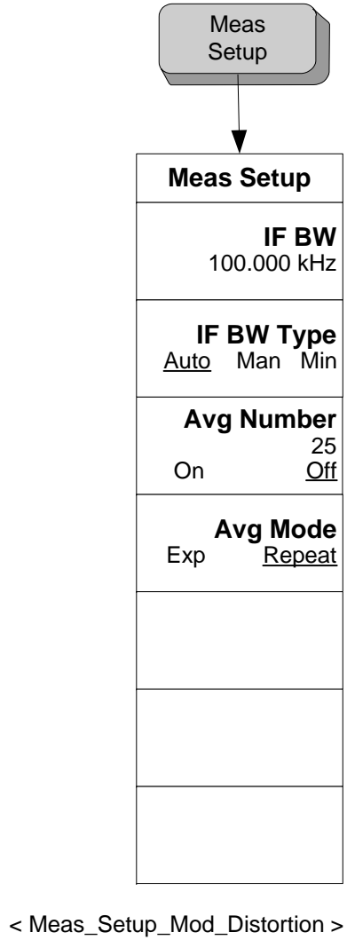
Figure 6-27 Modulation Distortion Measurement Setup Key Flow
