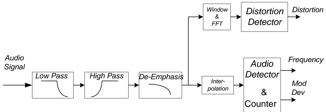
Figure 5-12 Audio Diagram
