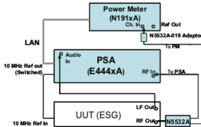
Figure 1-2 N5531S System Block Diagram
