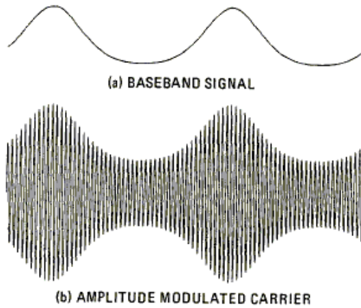
Figure 5-6 AM with an Asymmetrical Baseband Signal
