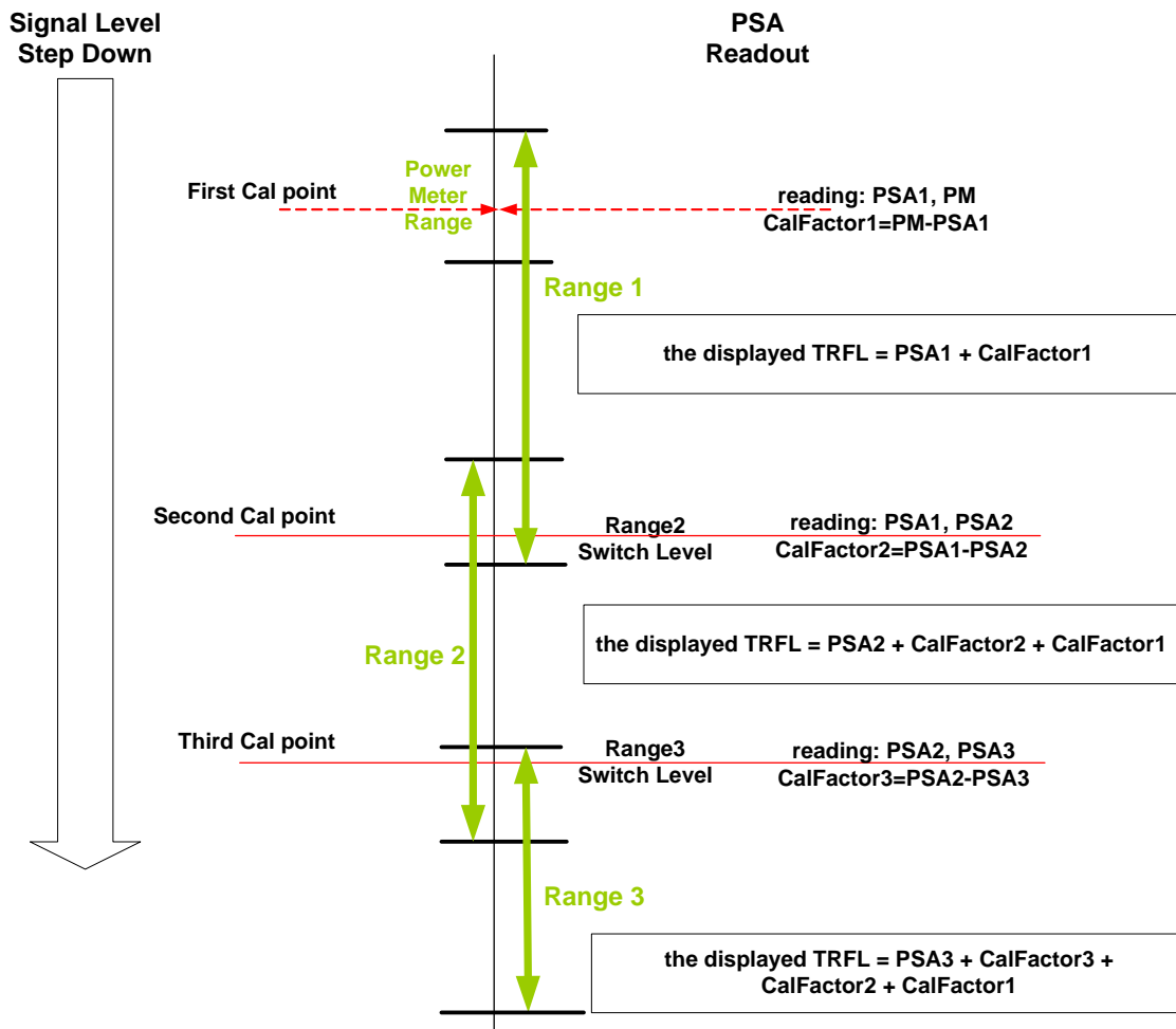
Figure 5-3 TRFL Ranging Calibration
