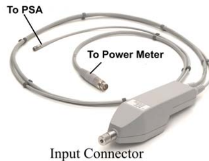
Figure 2-3 Connecting the Sensor Module to the UUT
